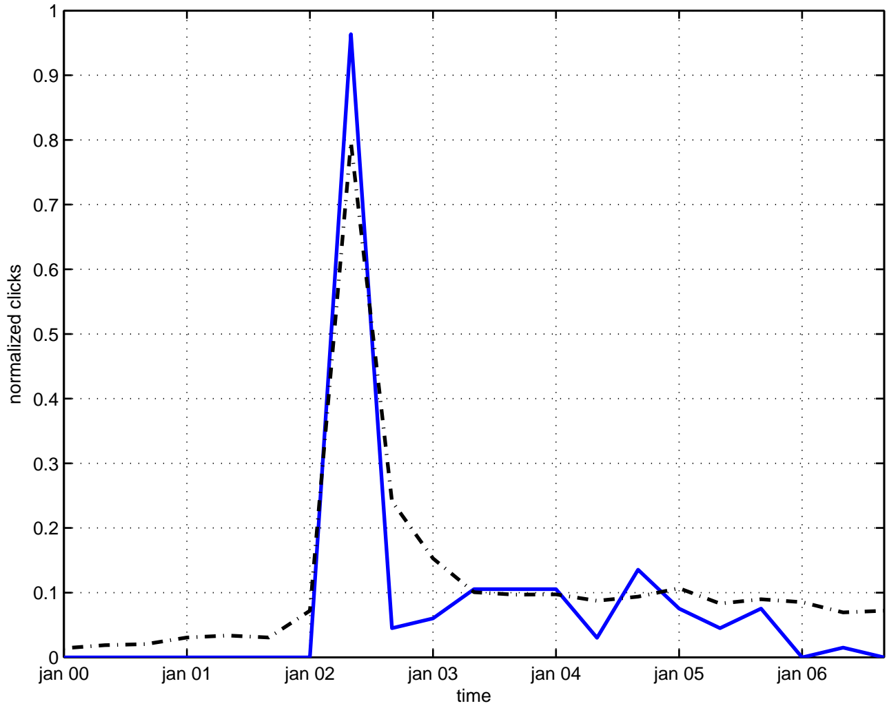
scalar symmetry
