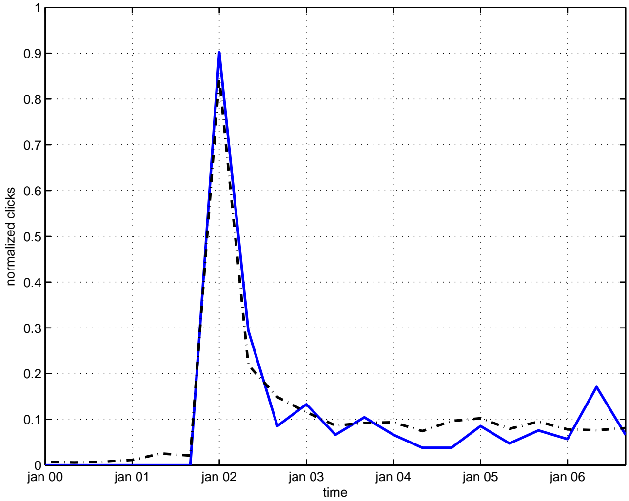
scalar solution
