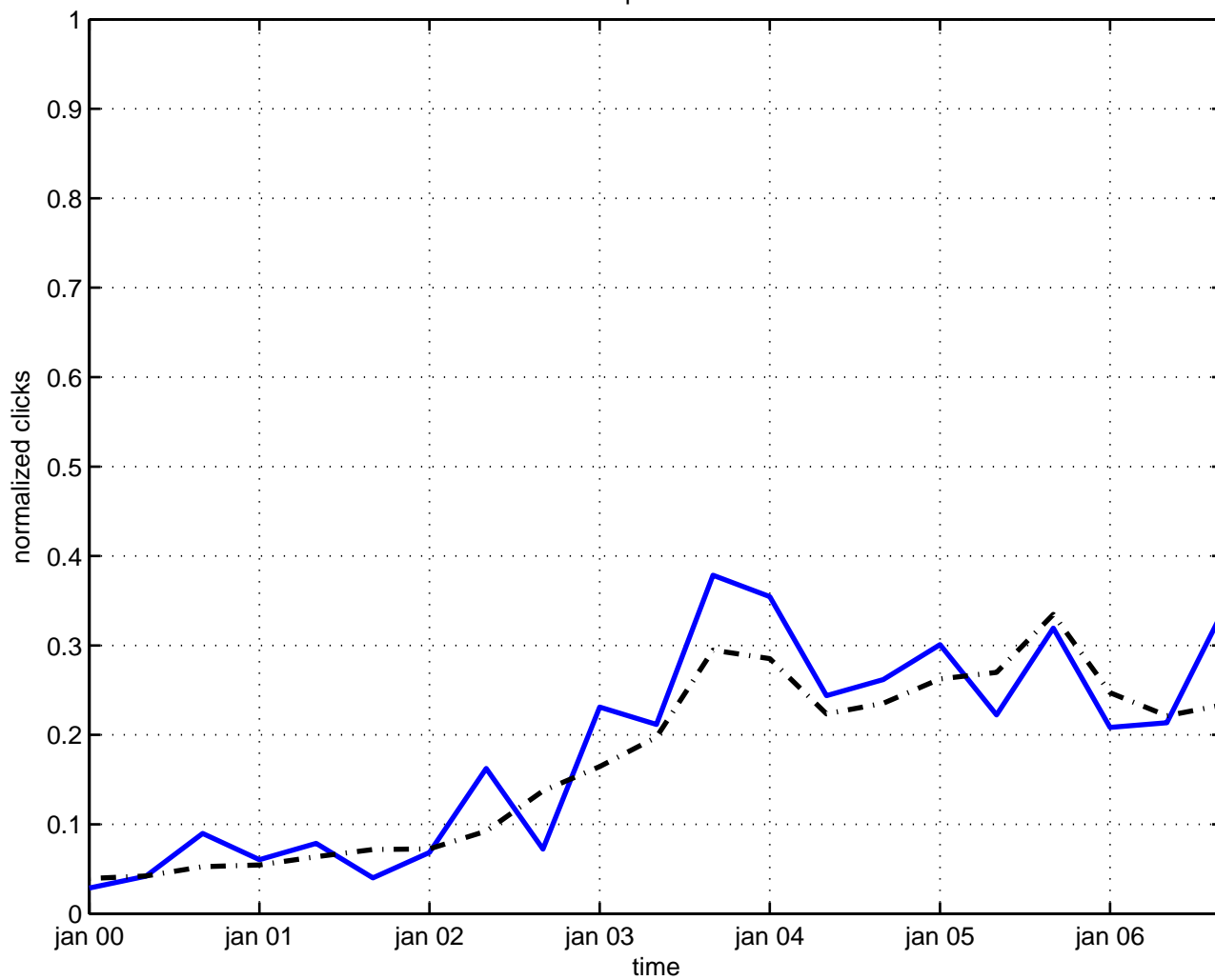
scalar perturbation
