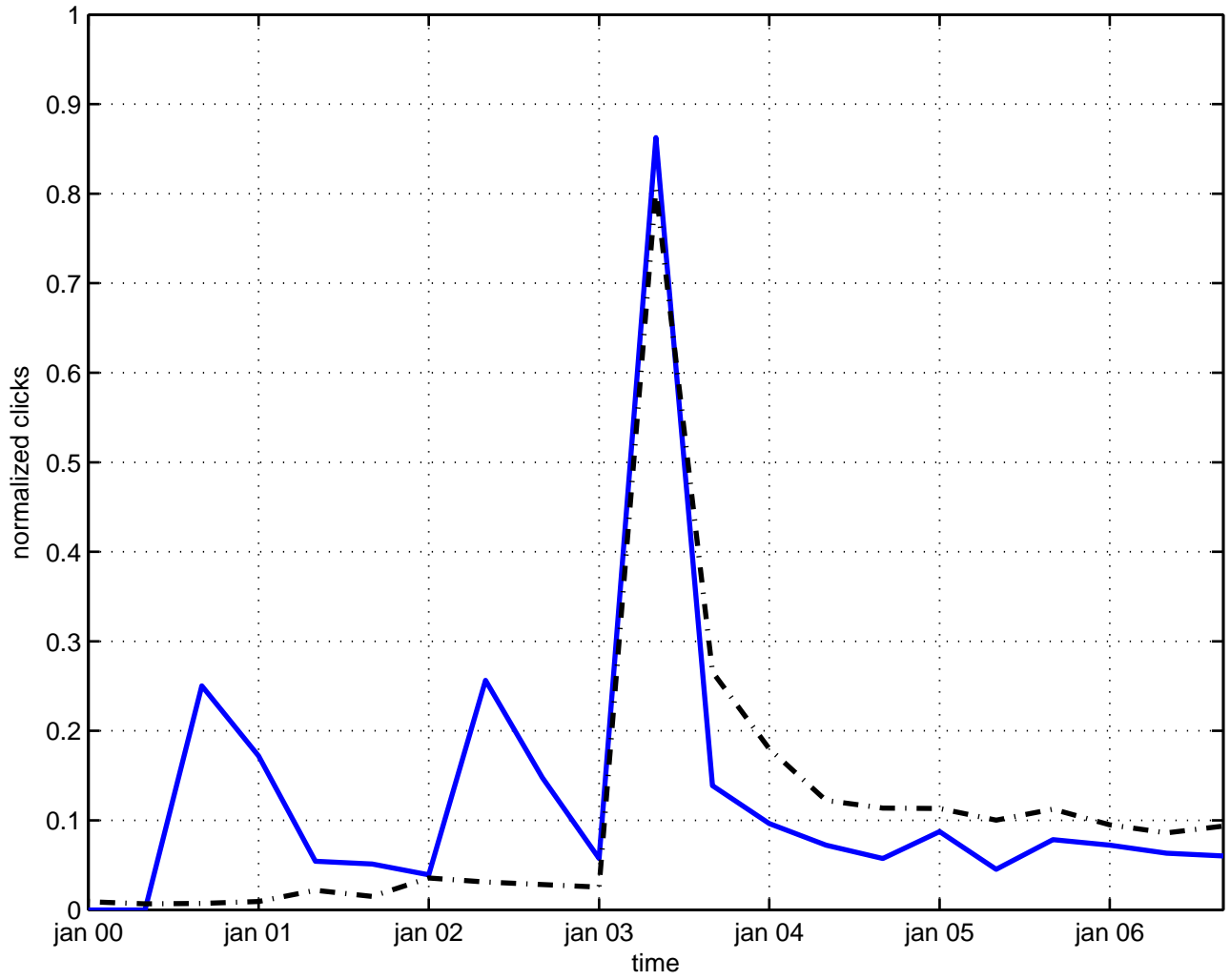
scalar multiplet
