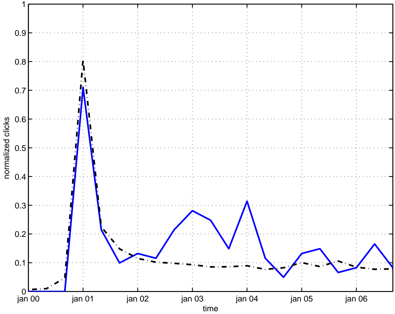
scalar gravitational radiation
