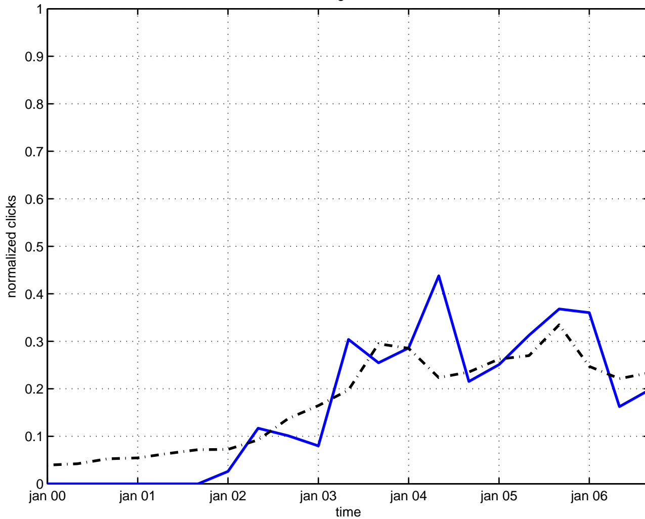
scalar gravitation
