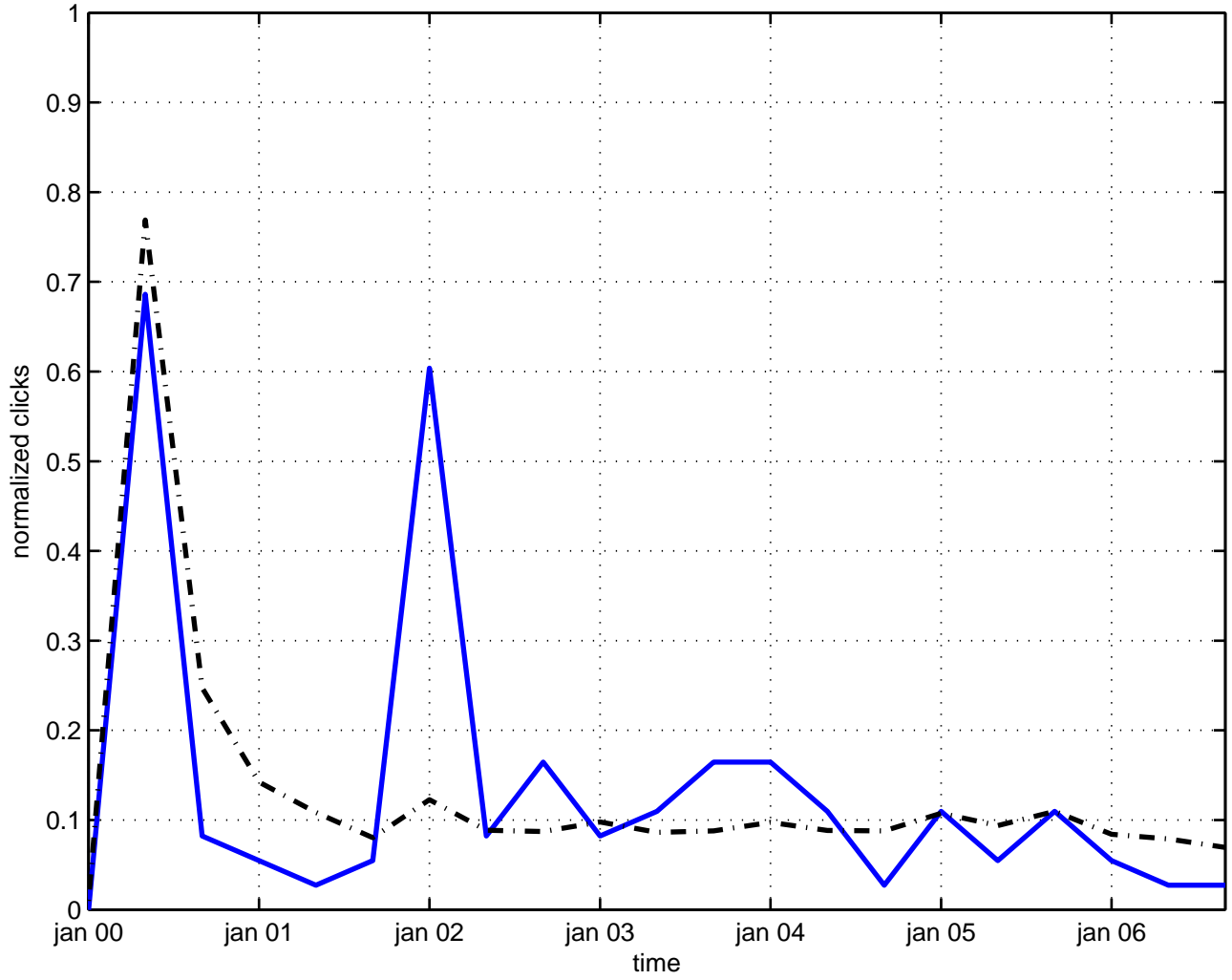
scalar field theoretical model
