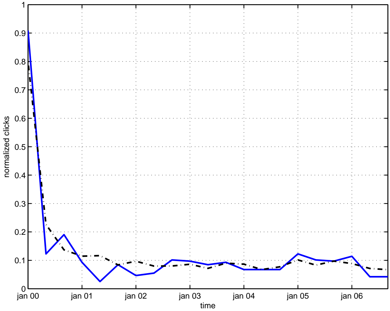
scalar exchange
