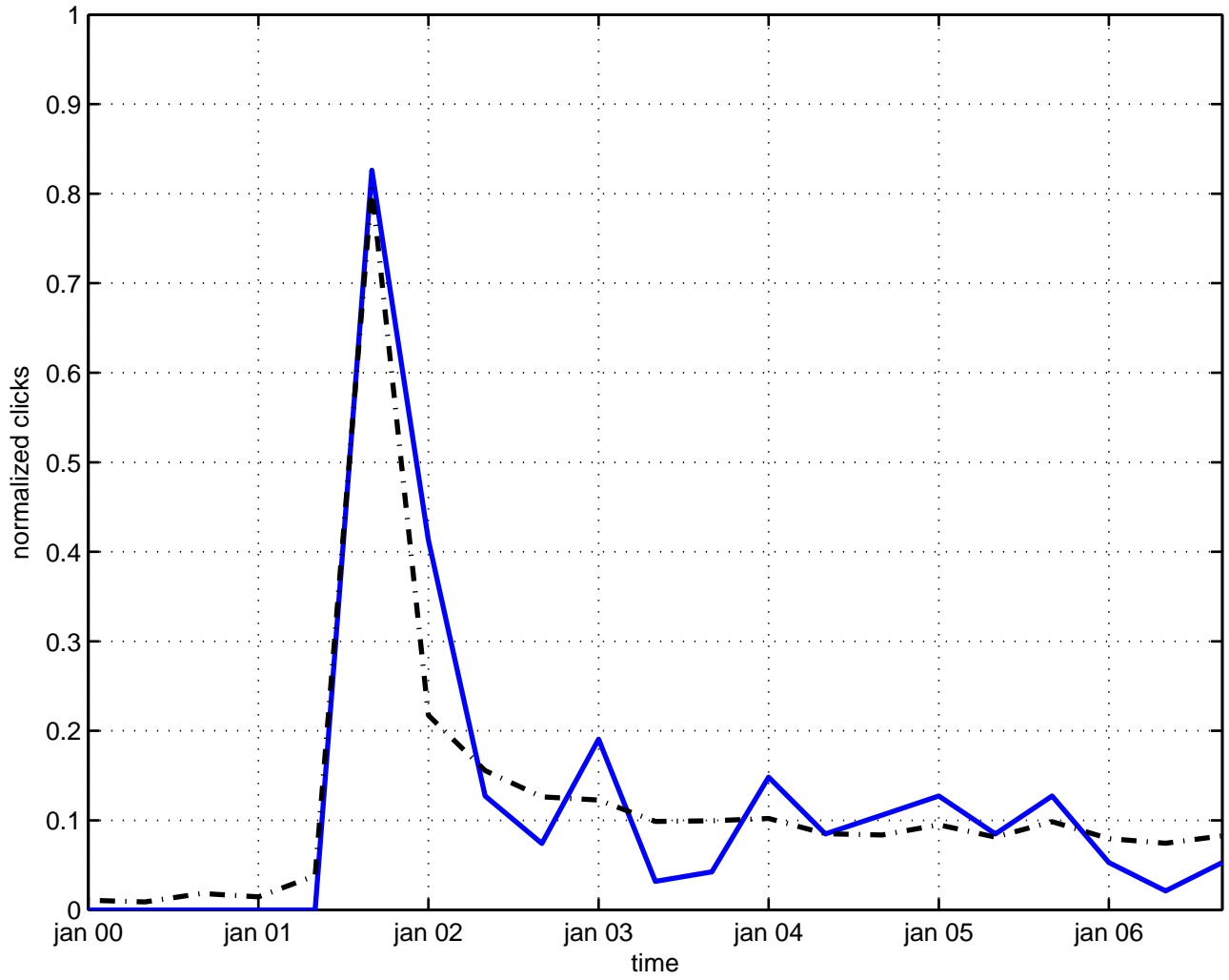
scalar doubleton
