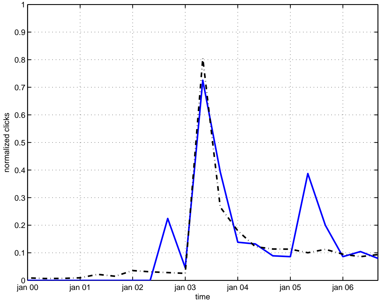
scalar coupling
