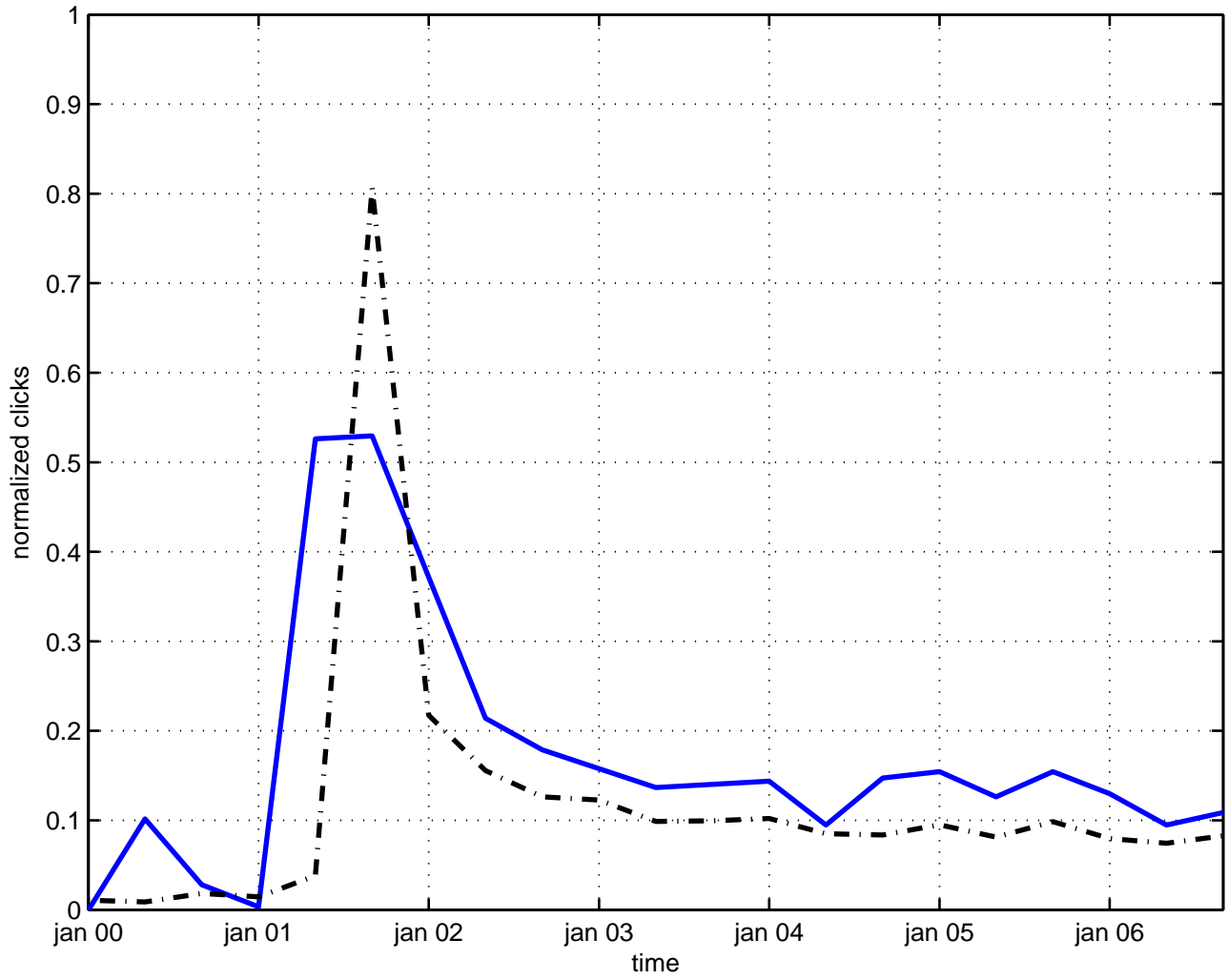
scalar bound state
