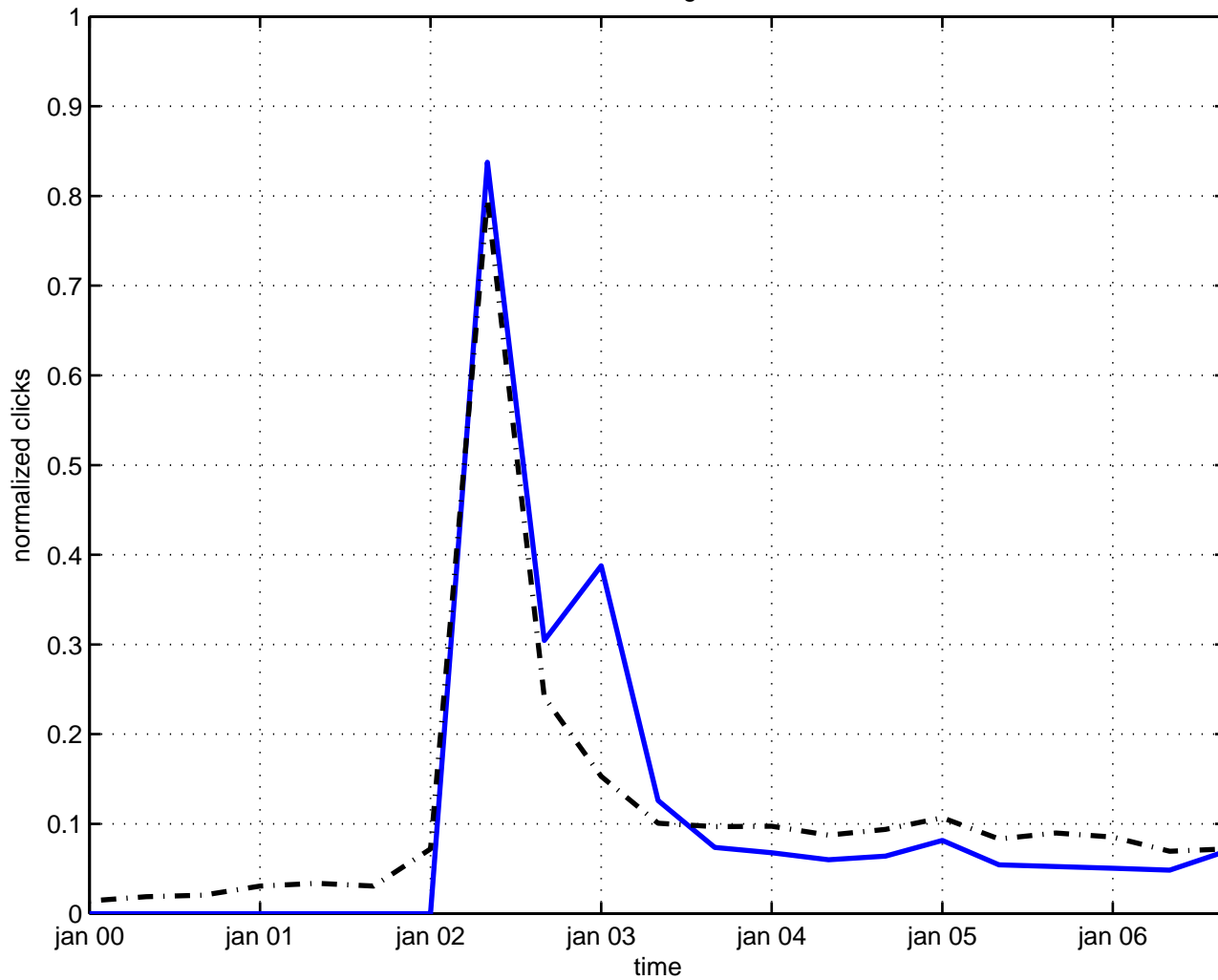
scalar background
