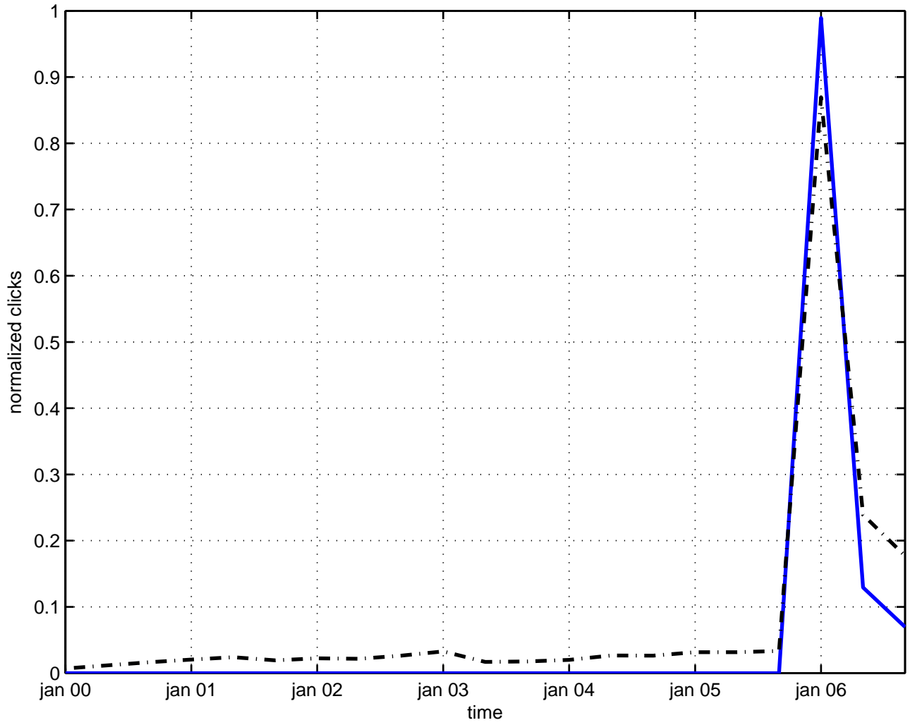
sagnac effect
