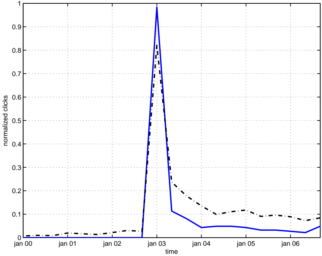
s0(1,10) invariance
