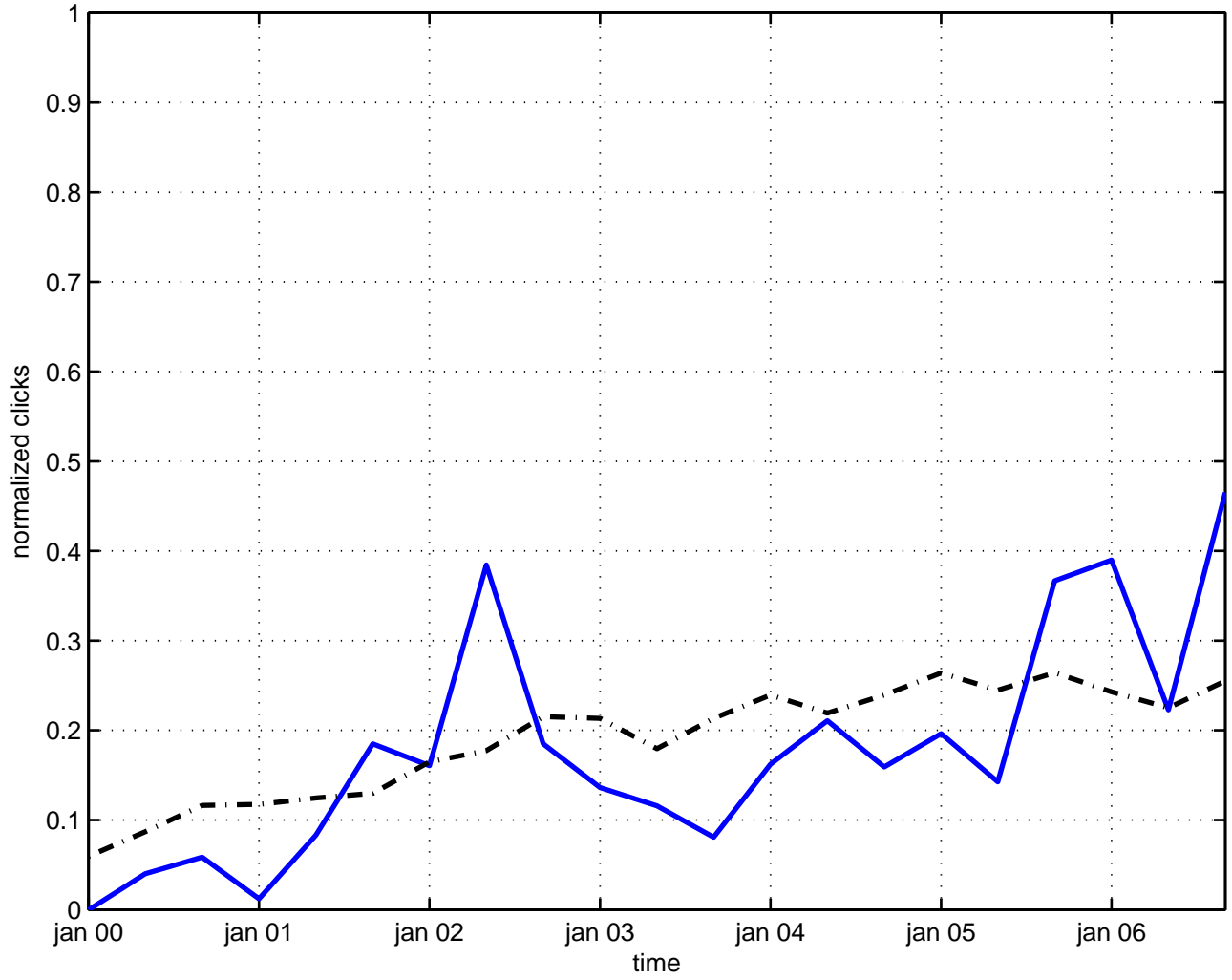
s-duality
