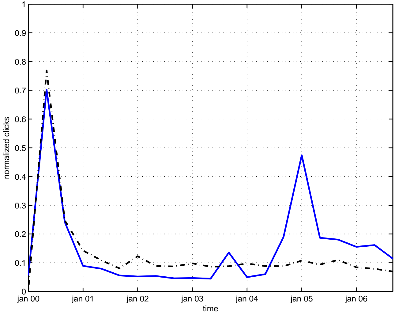
s-duality duality
