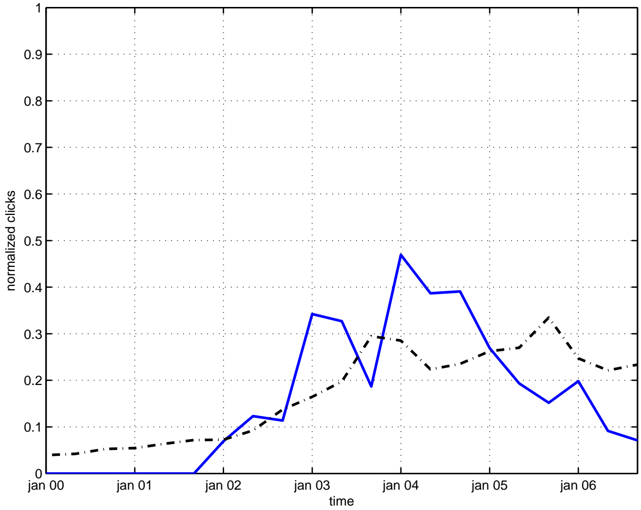
s-brane membrane model
