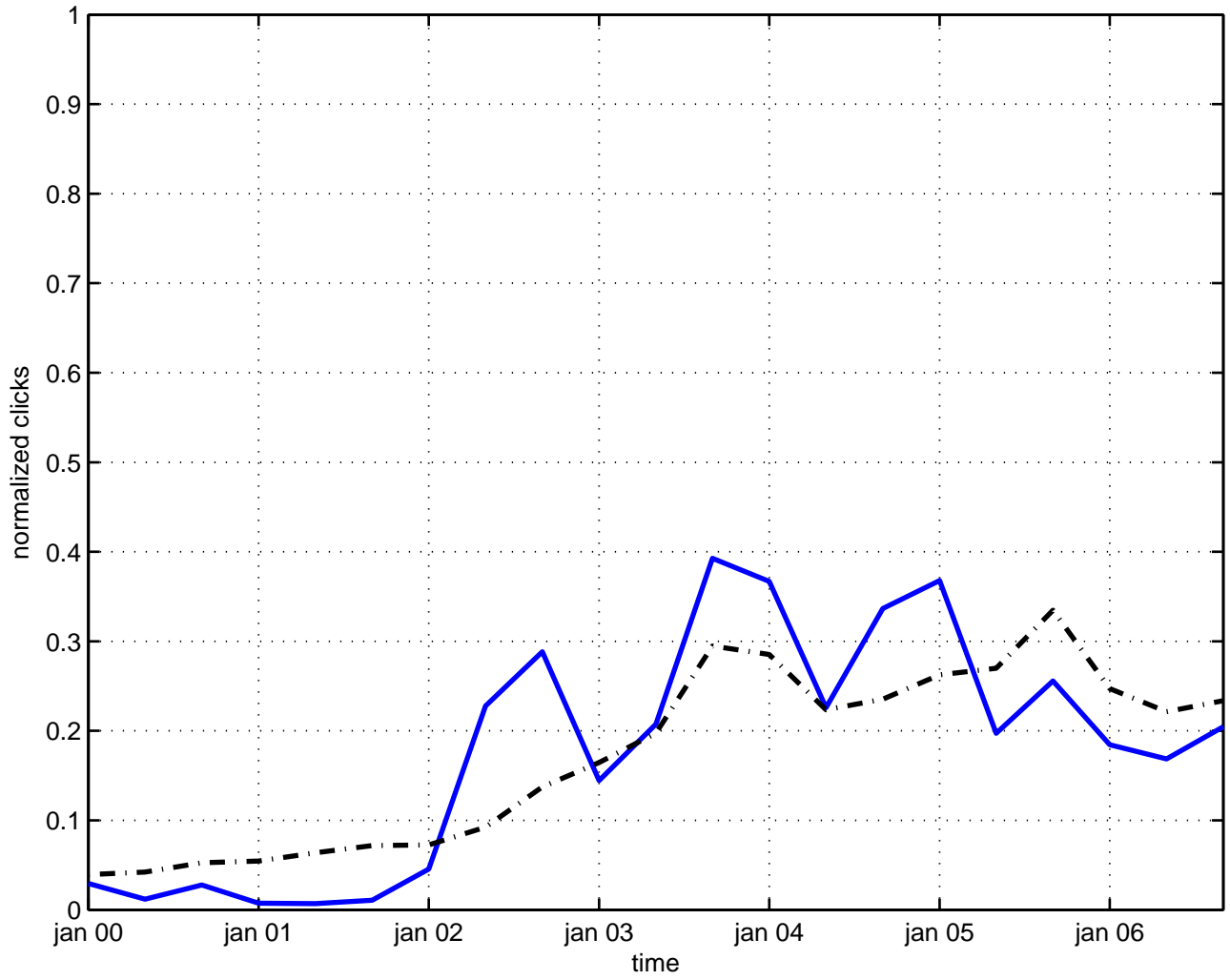
s(5) space-time
