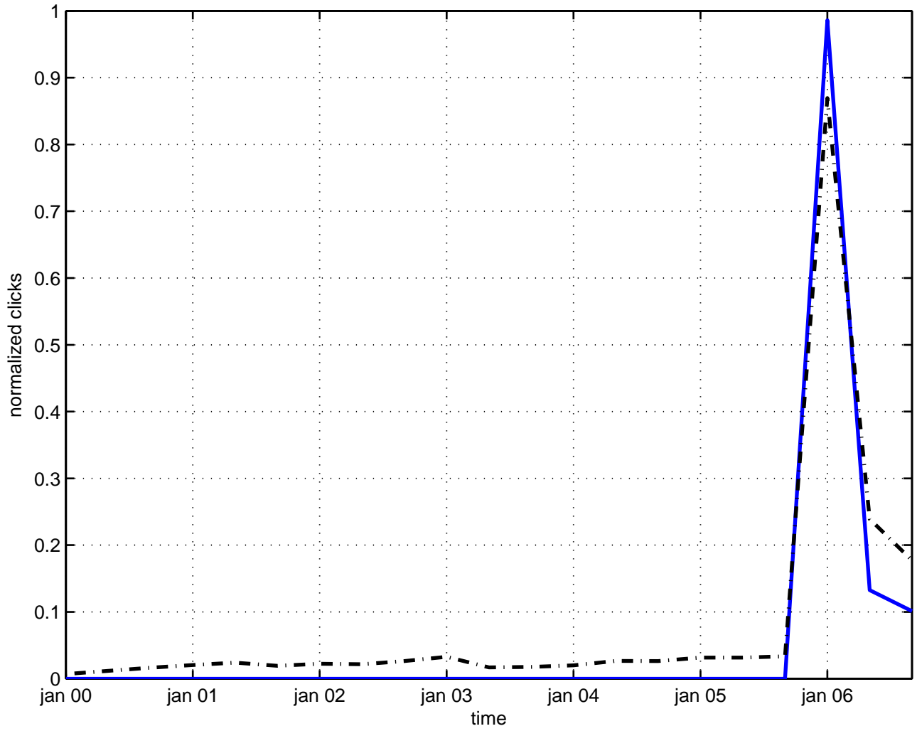
s(3) x r space-time
