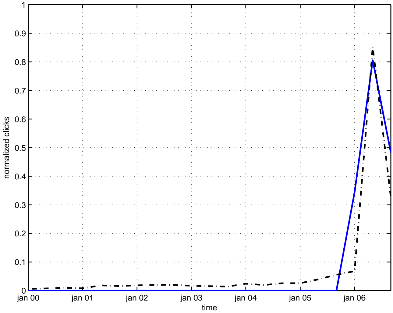
s(3) x r(1) space-time
