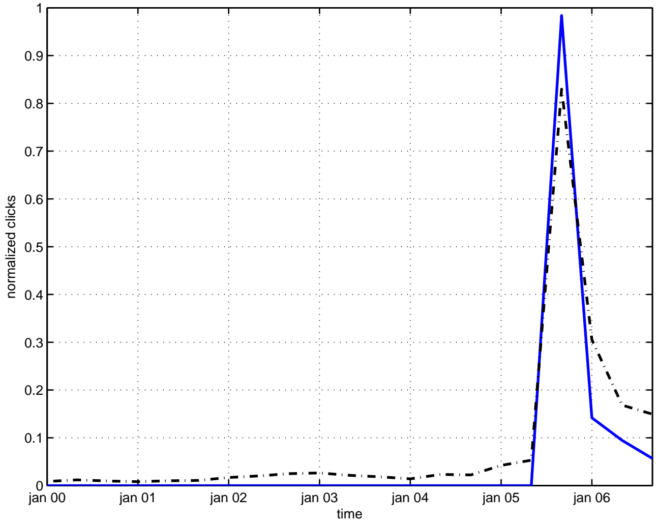
s(3) symmetry
