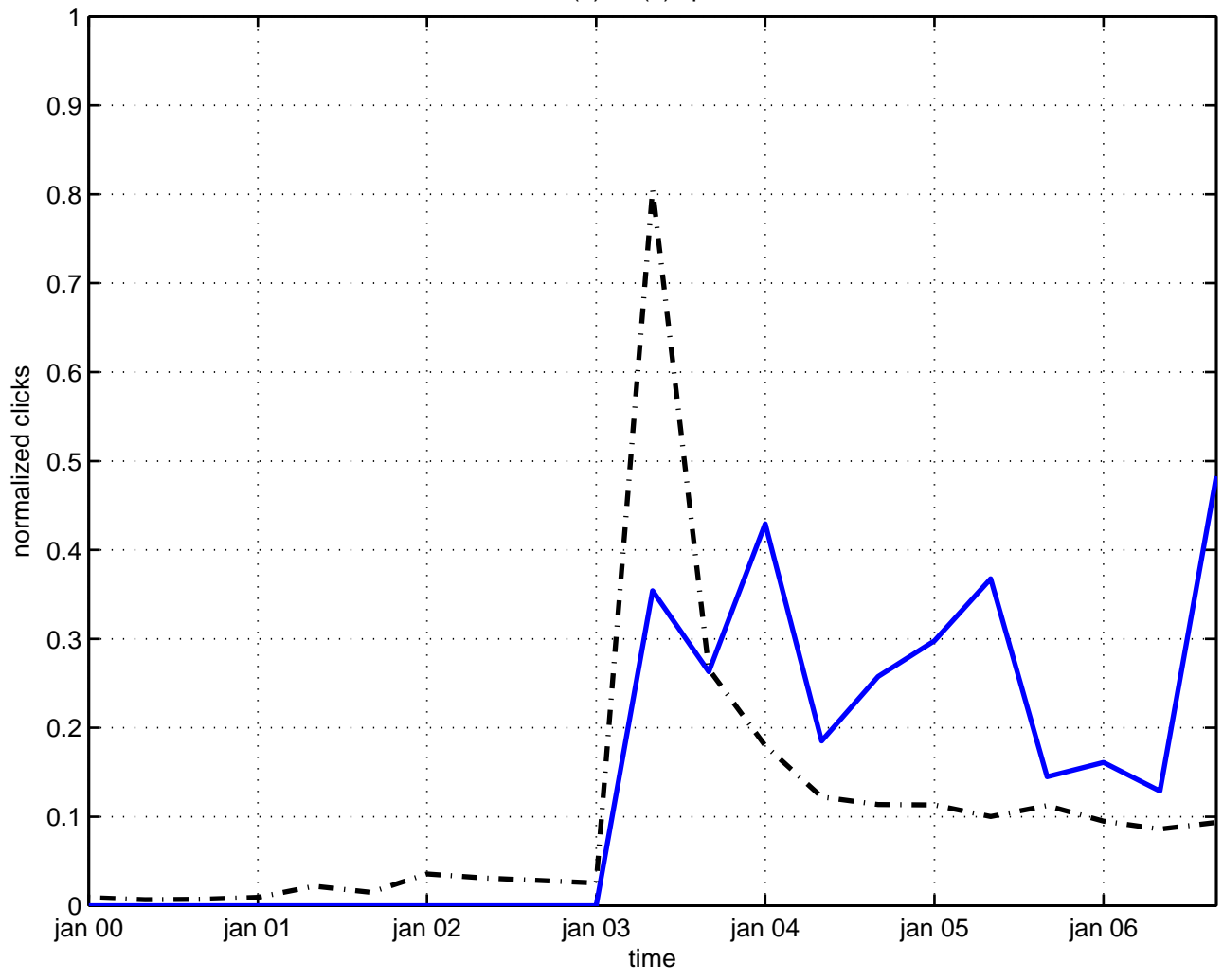
s(2) x s(2) space
