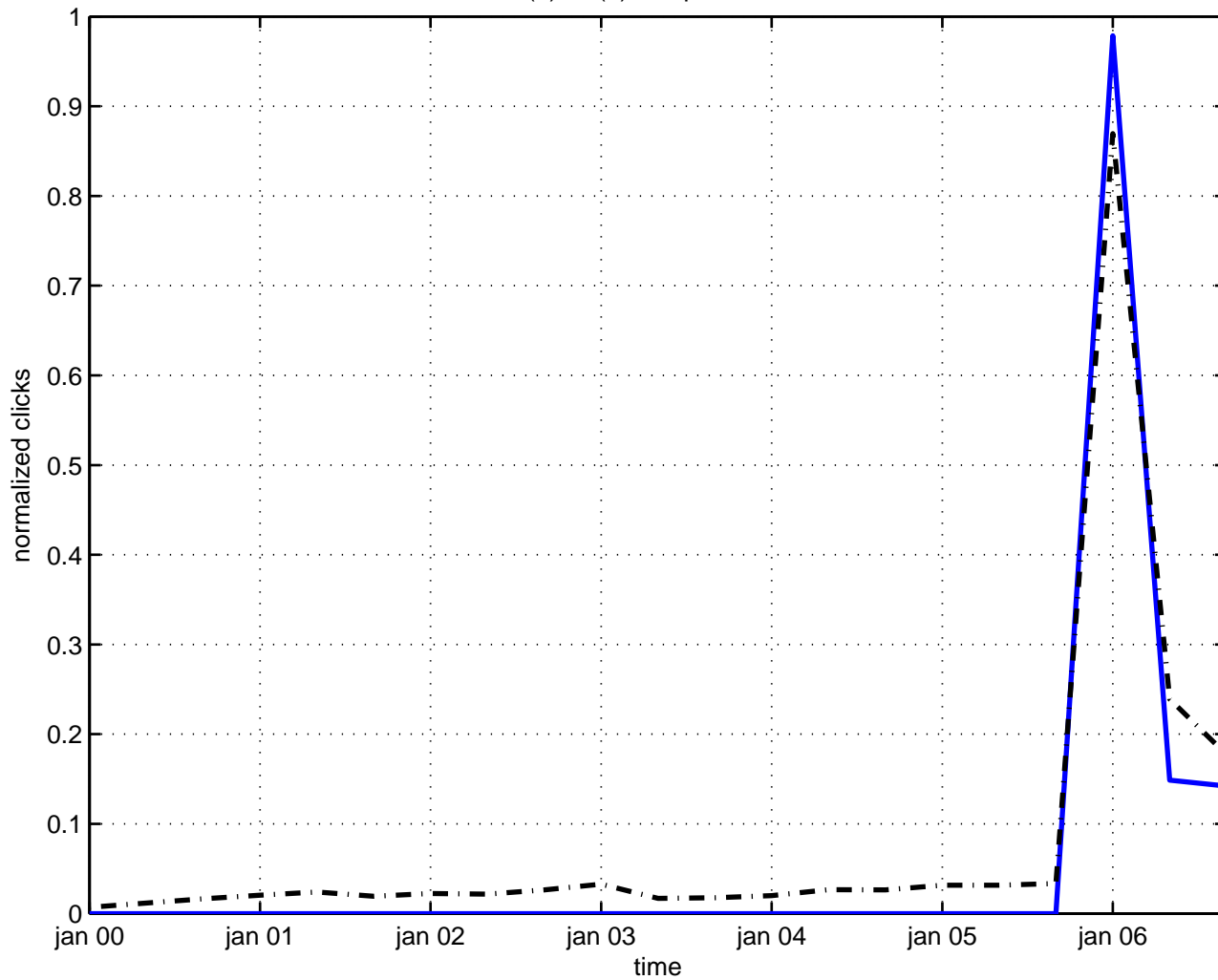
s(2) x s(1) x r space-time
