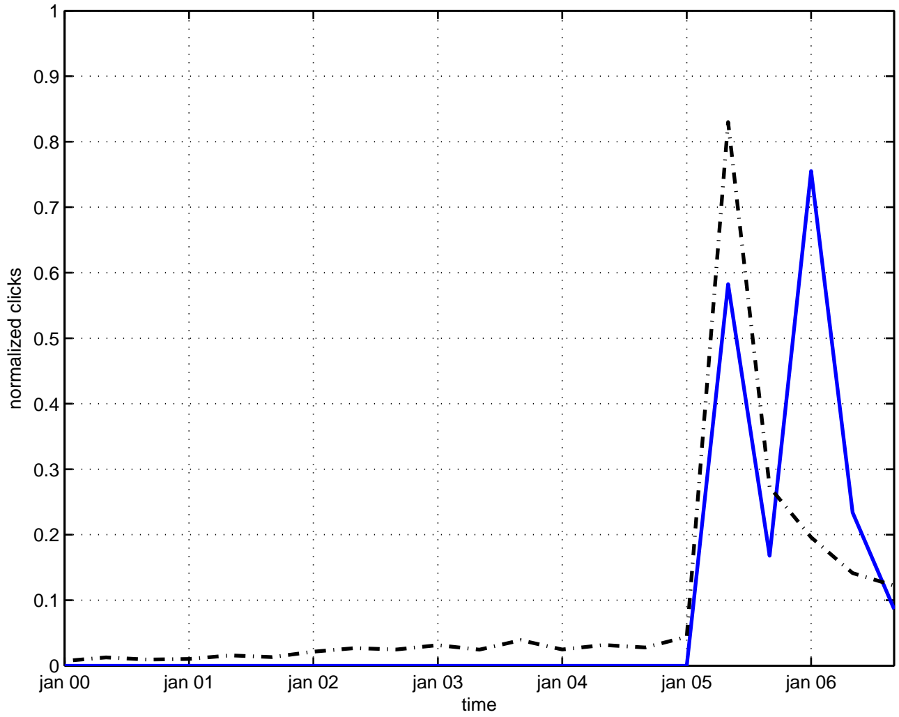
s(2) compactification
