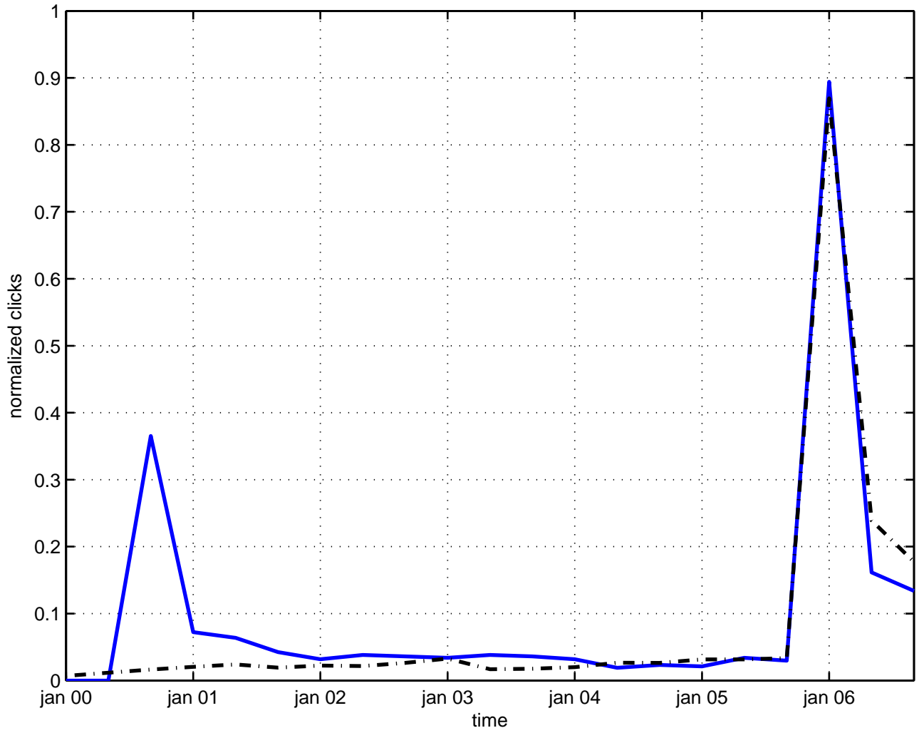
s(1)/z(2) space
