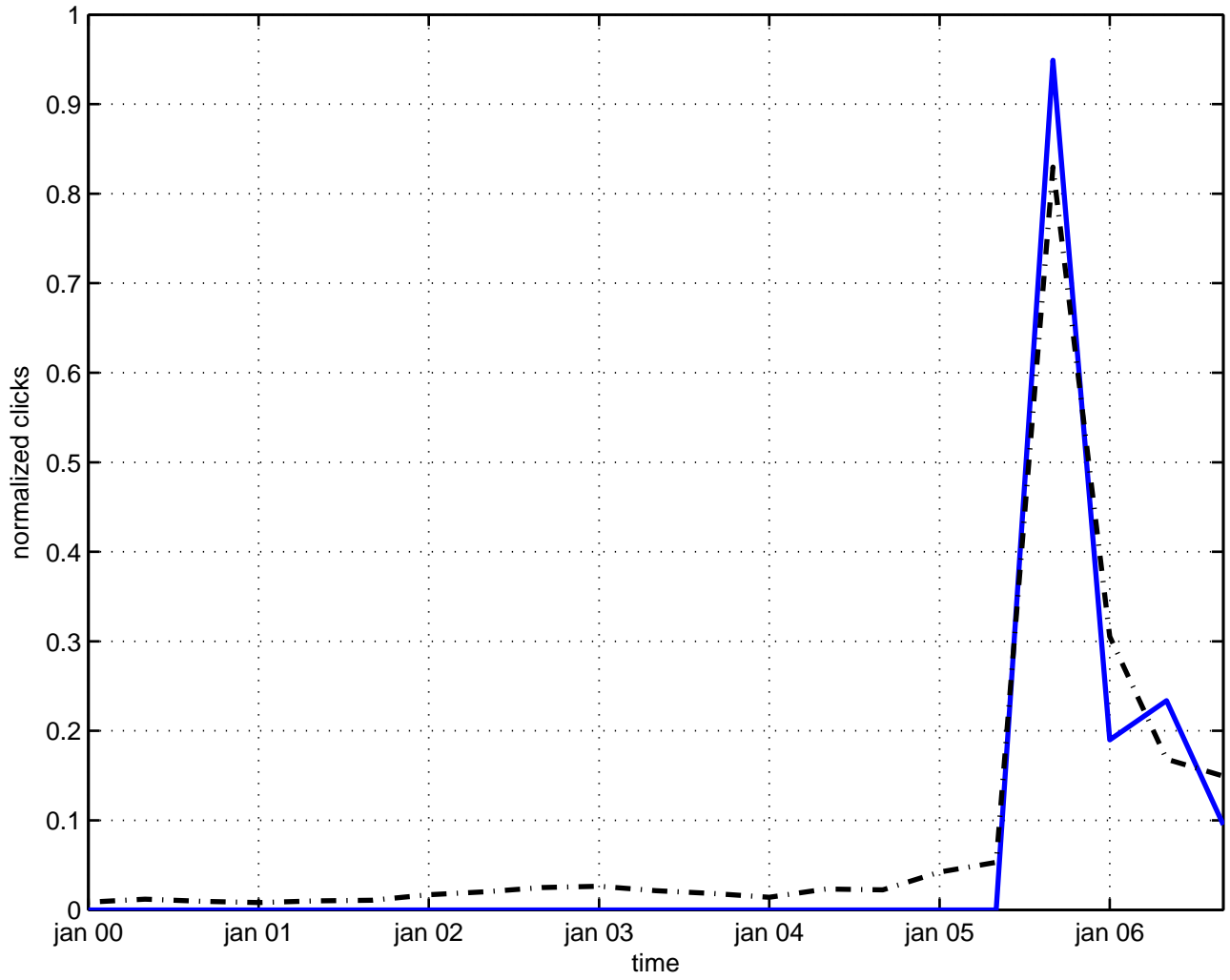
s(1)/t(1) space
