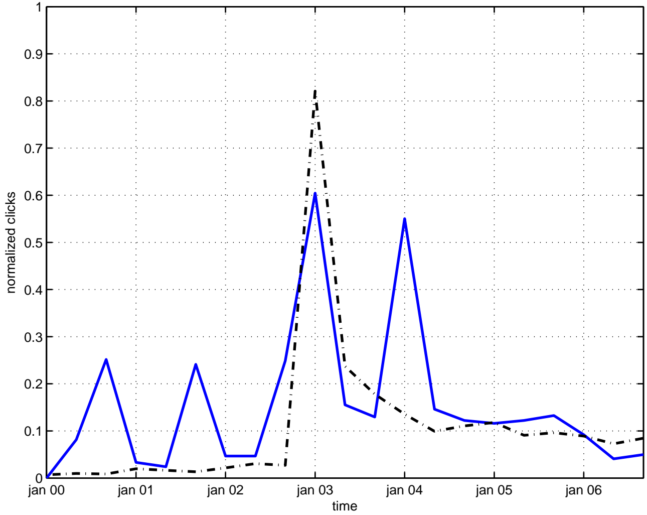
s(1) spontaneous compactification
