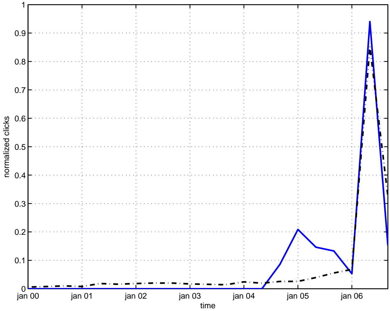
s(1) compactification
