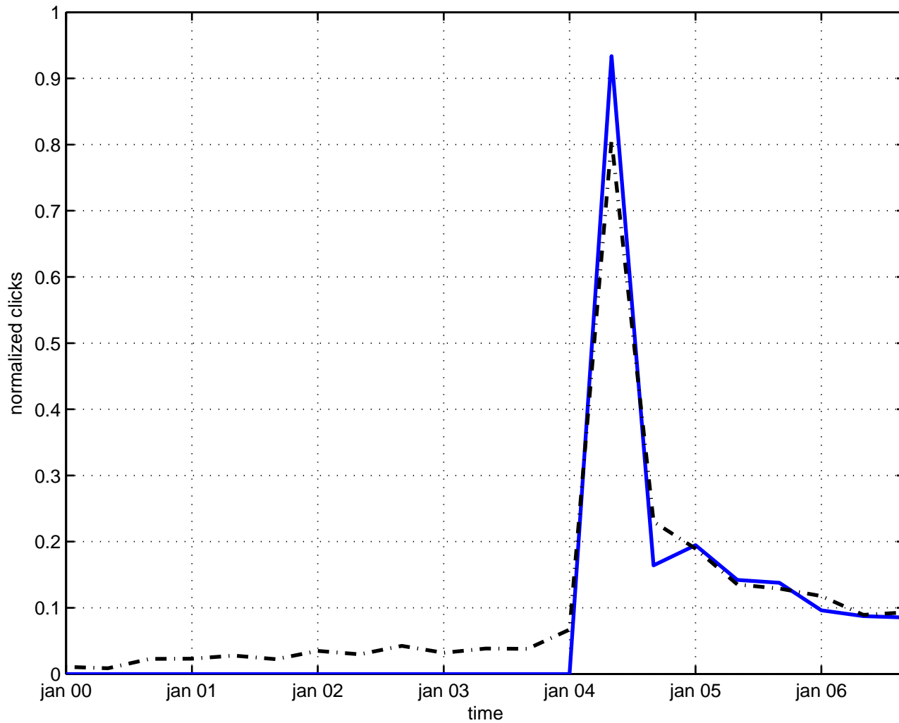
rubakov-callan effect
