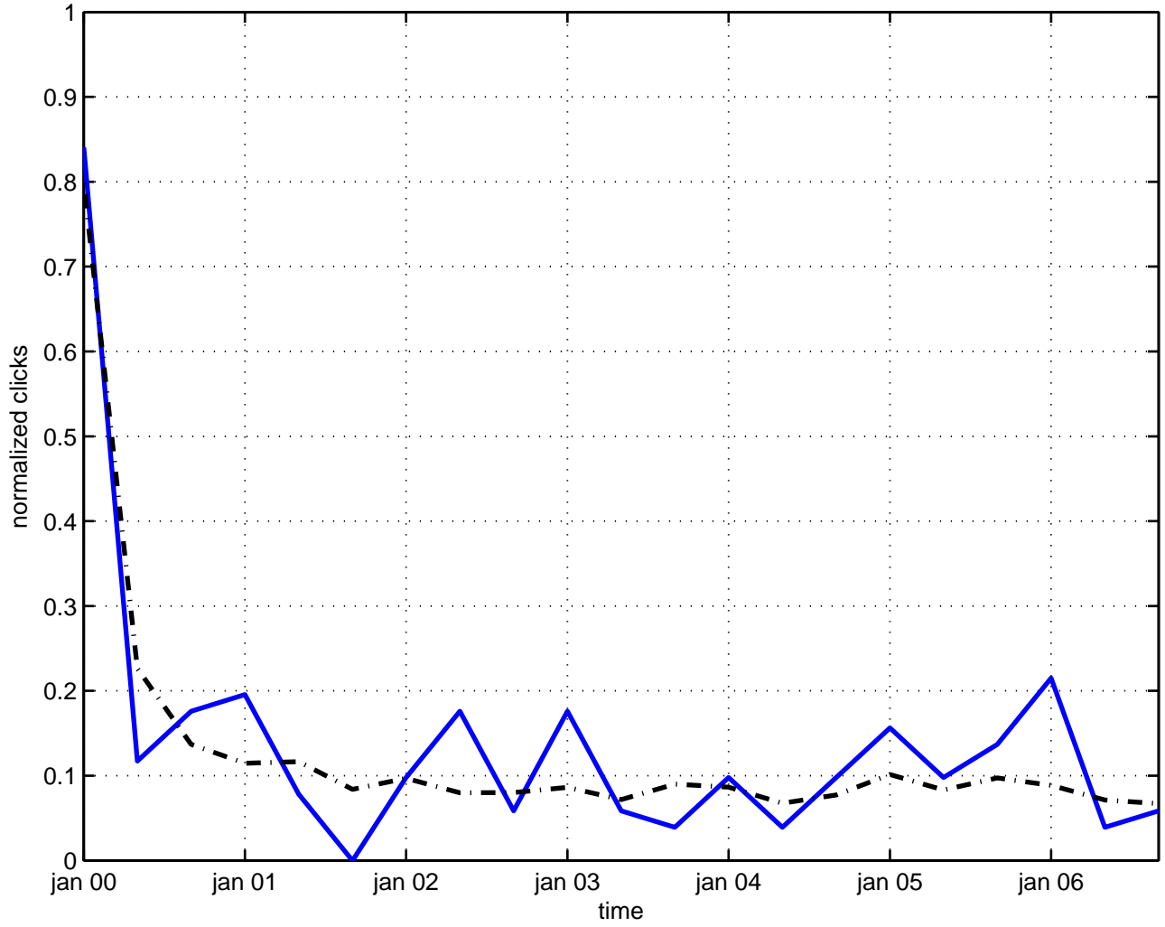
rp(2) field theory
