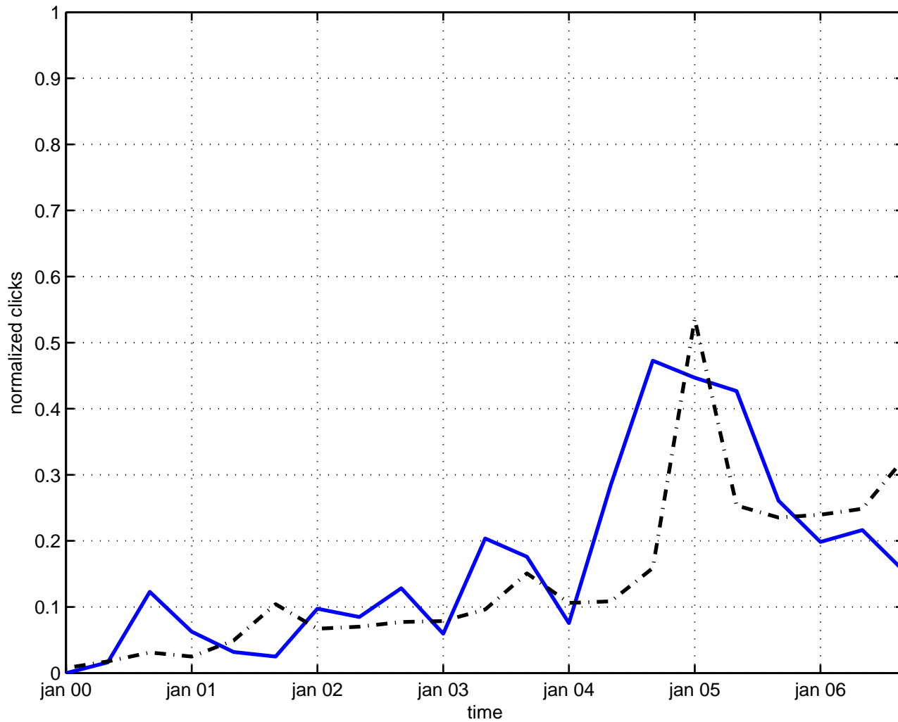
rotator black hole
