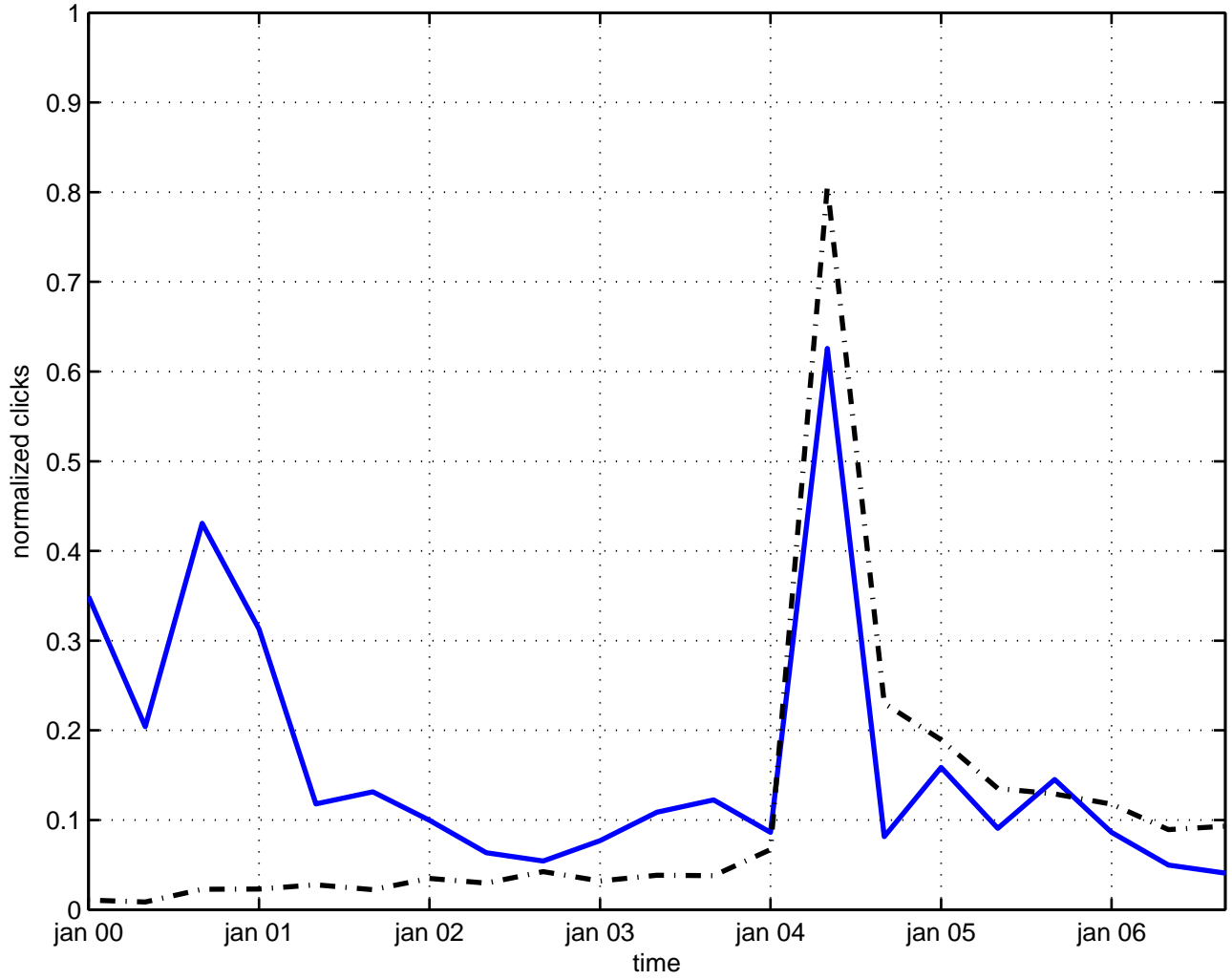
rotational invariance
