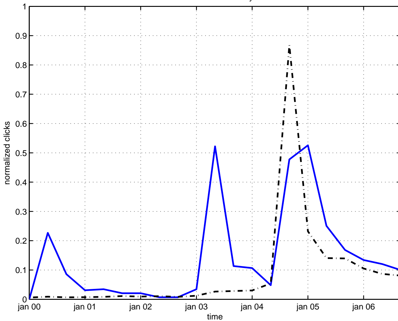
rotational field theory
