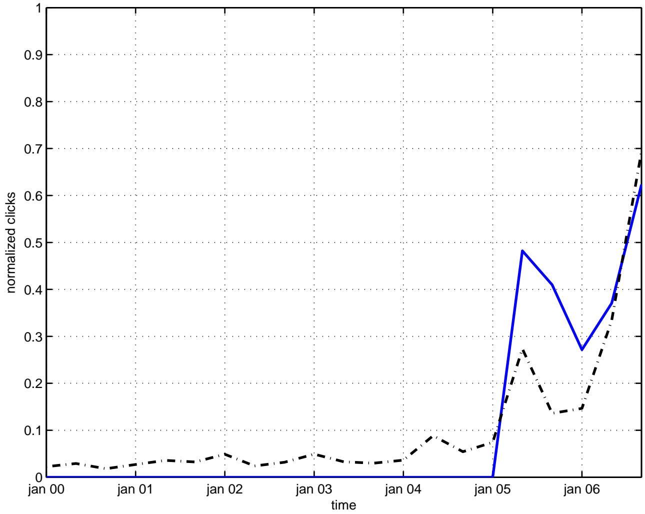
rotation symmetry
