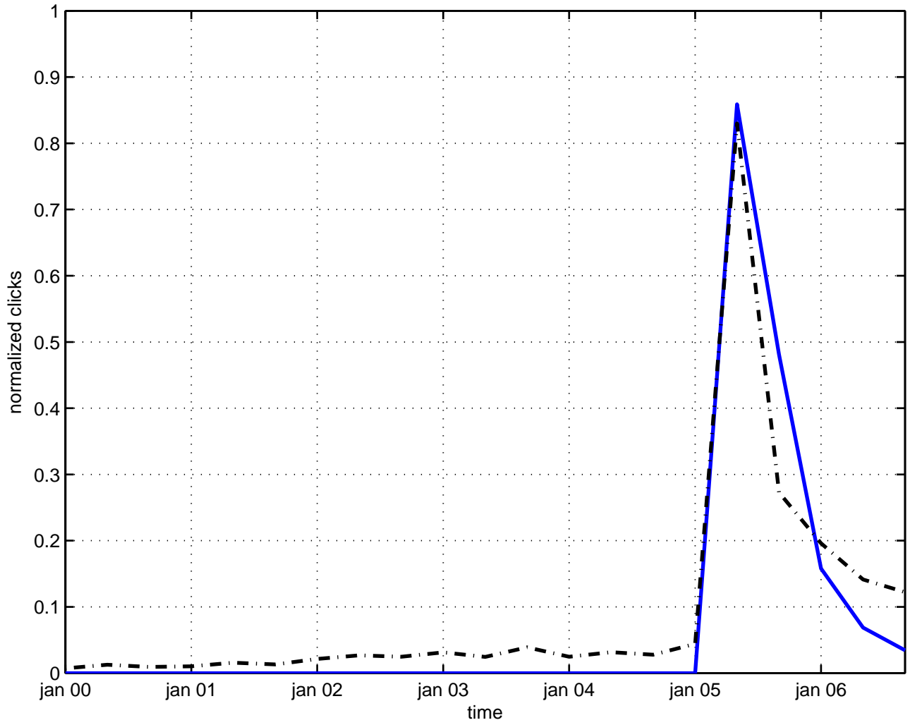
rotation polarization
