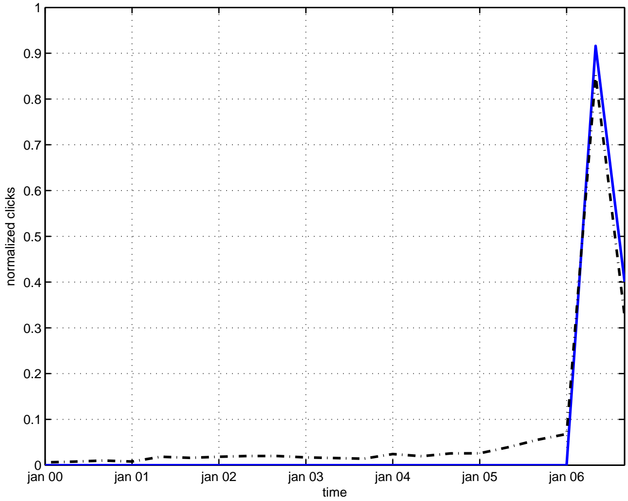
rotation attractor
