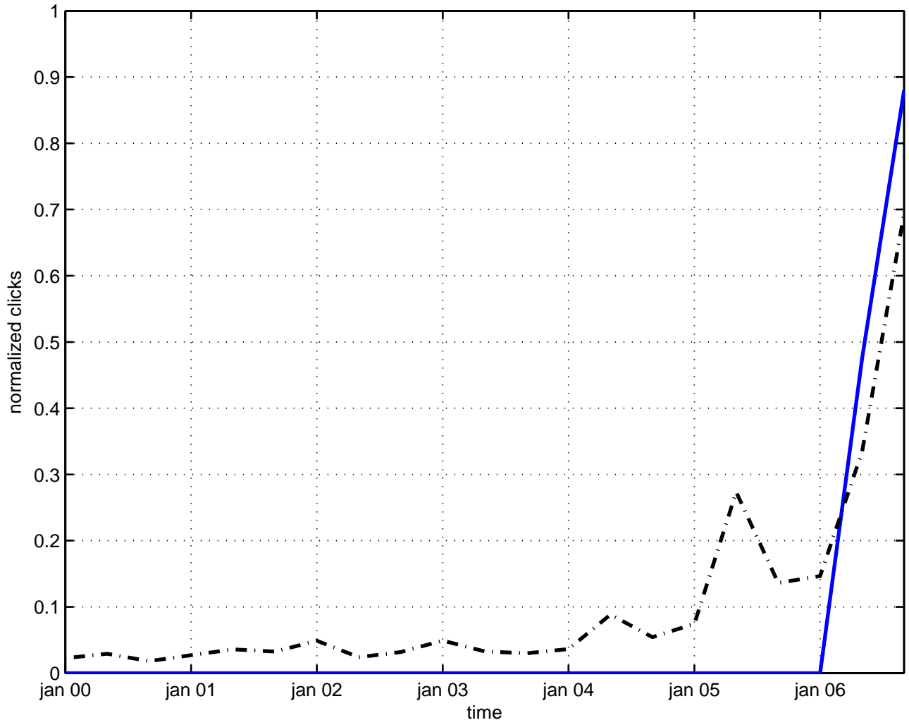
ricci flow
