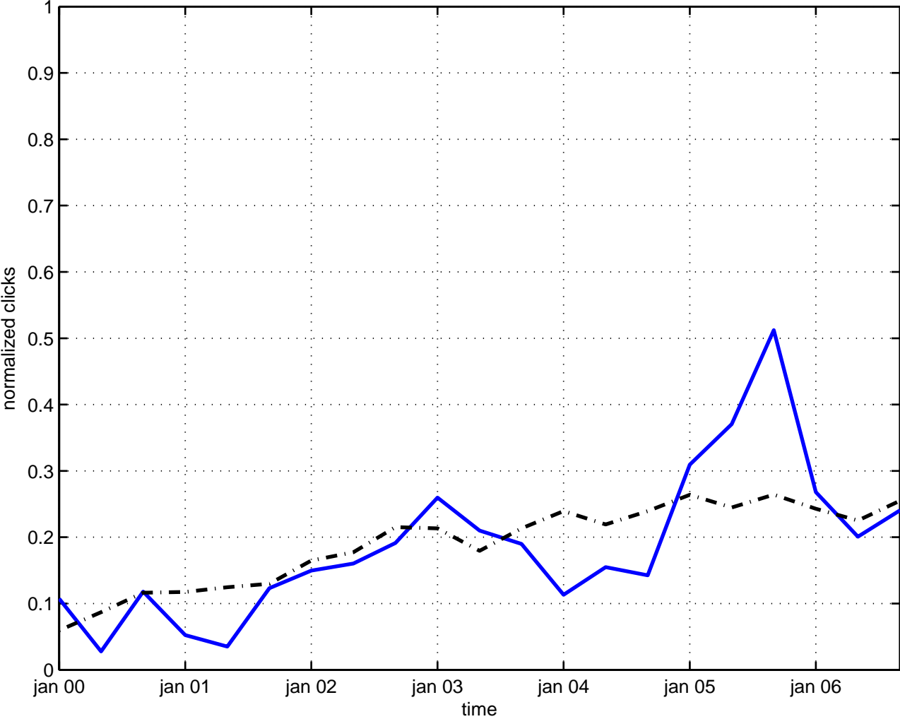
representation supersymmetry
