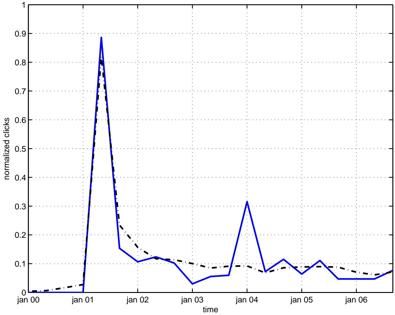
representation renormalization group
