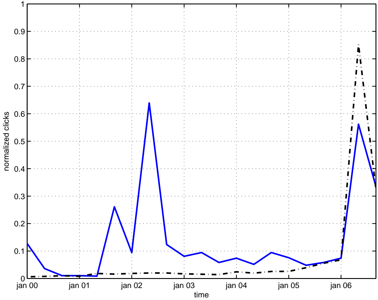
representation current algebra
