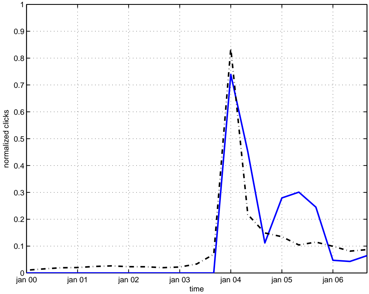
renormalization riccion
