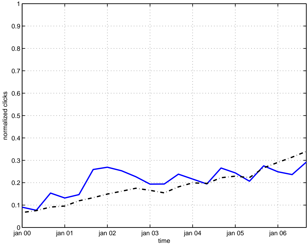
renormalization group
