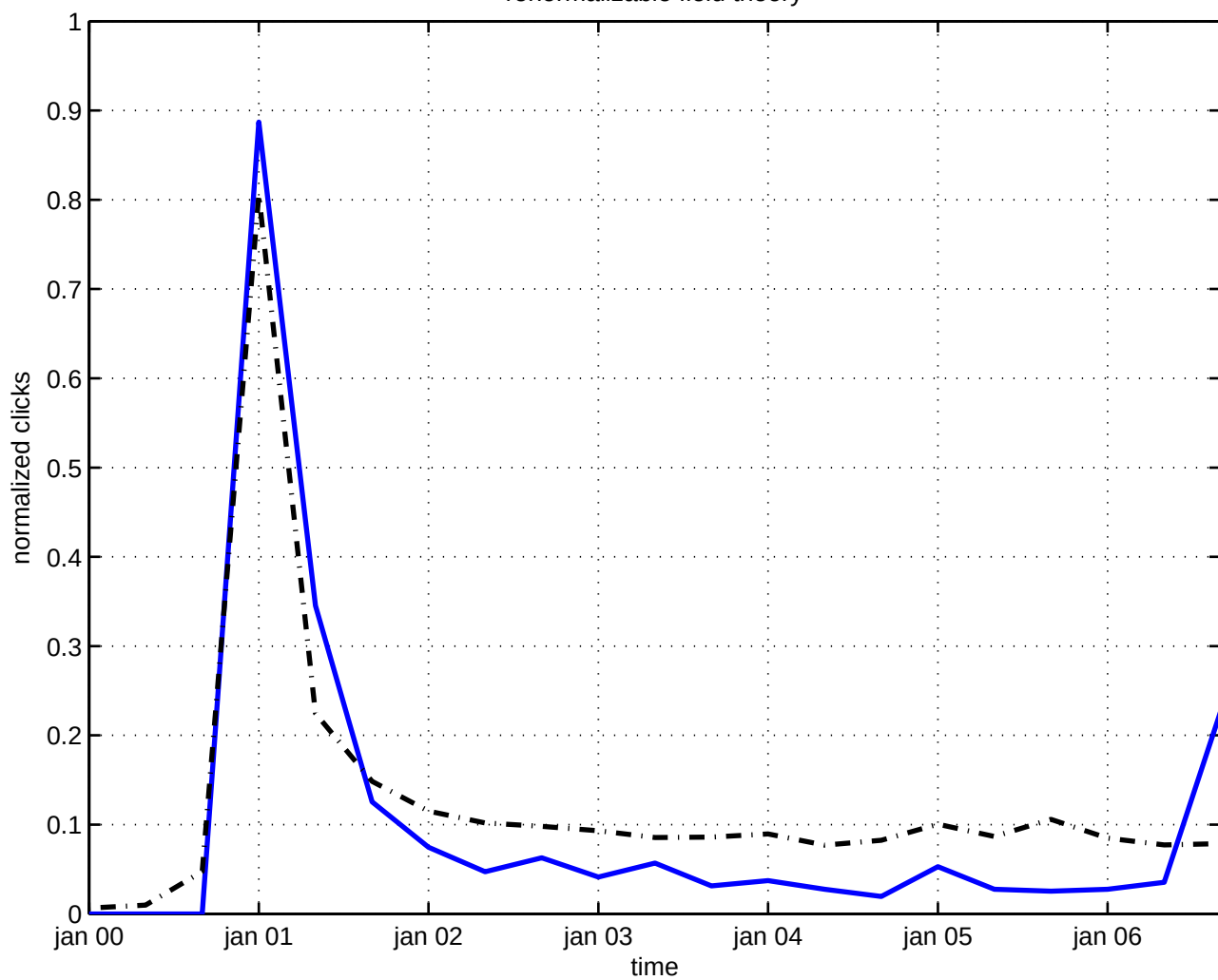
renormalizable field theory
