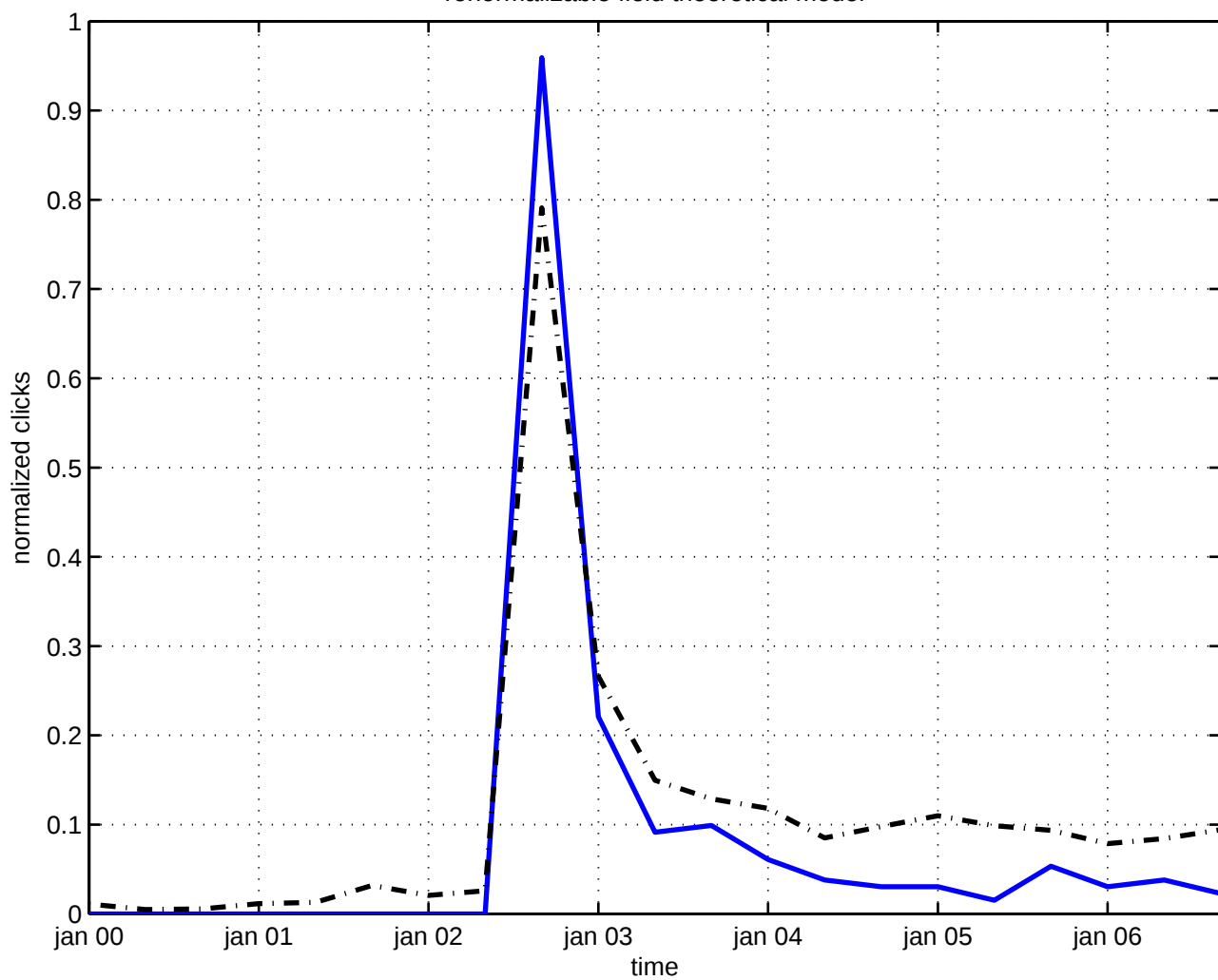
renormalizable field theoretical model
