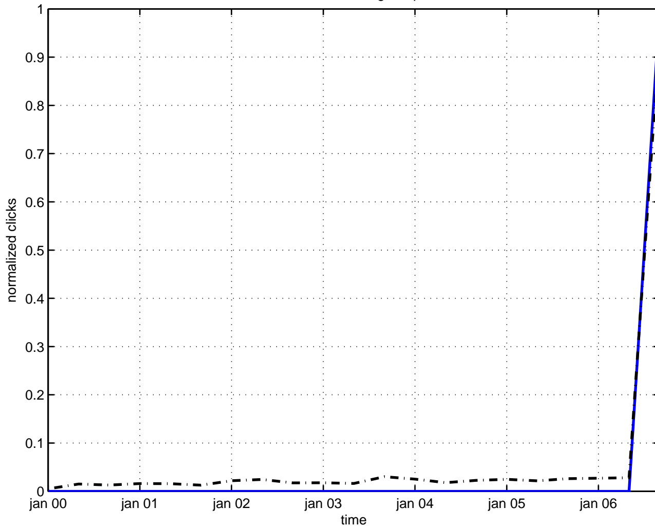
relativistic schroedinger equation
