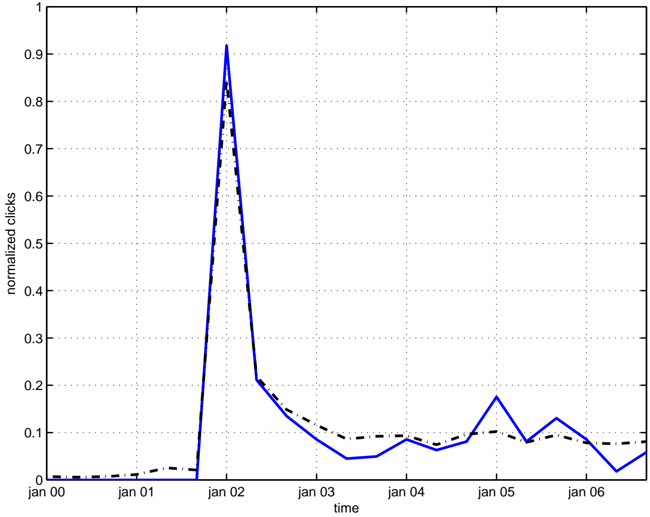
relativistic potential
