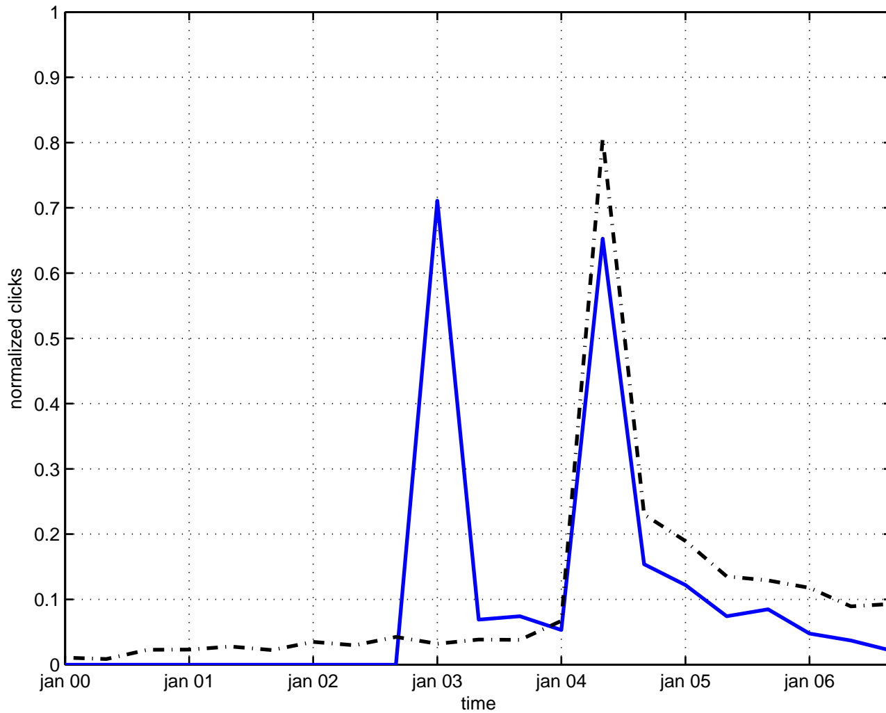
relativistic mechanics
