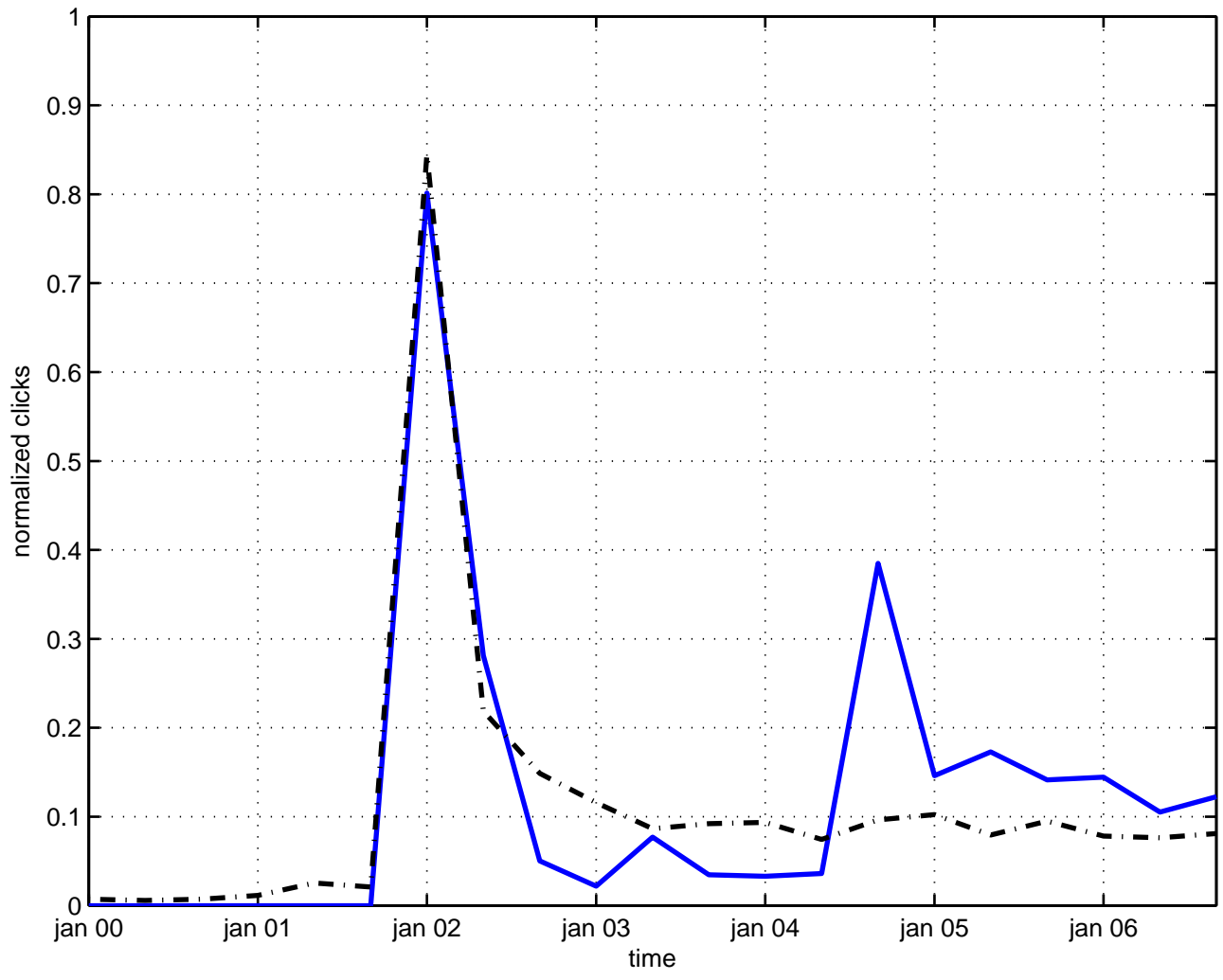
relativistic invariance
