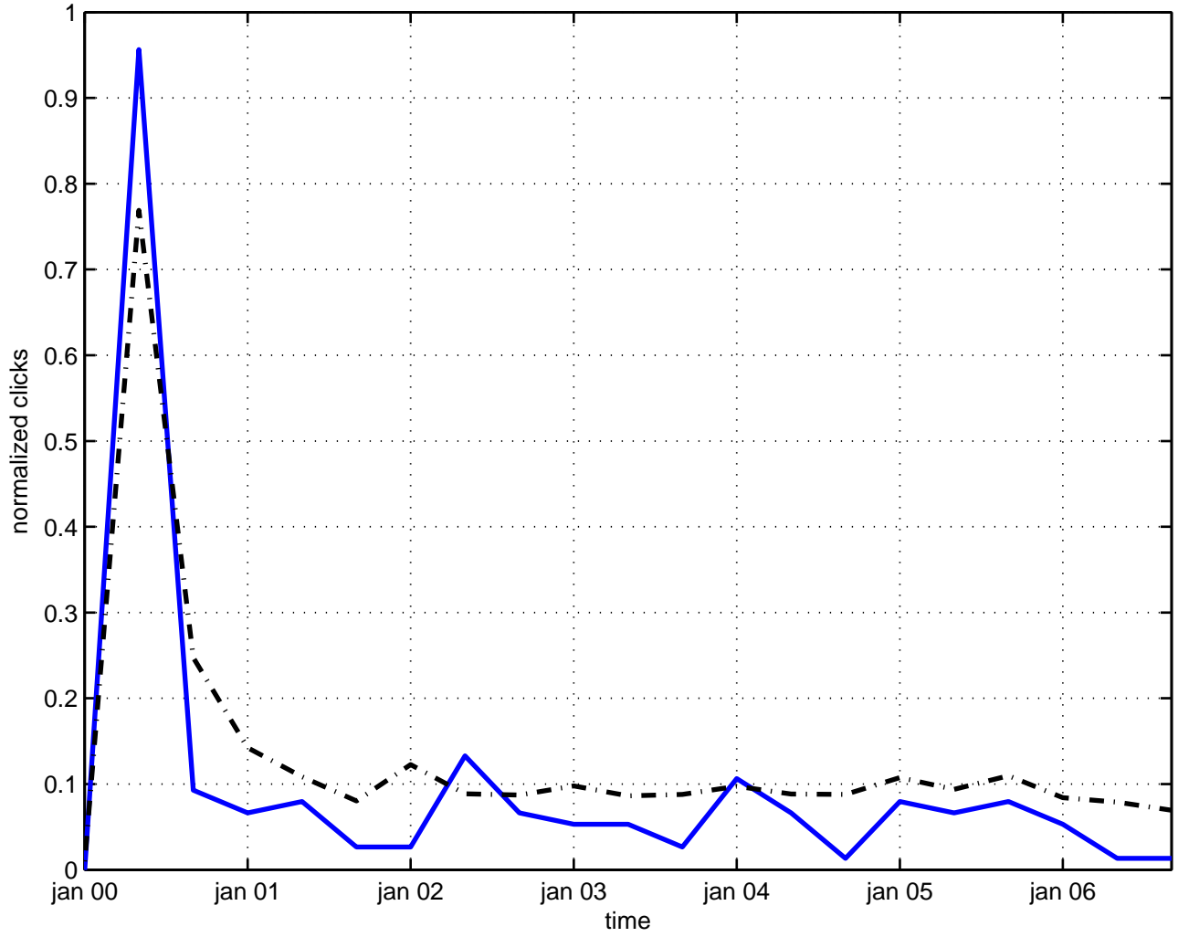
relativistic fermi gas
