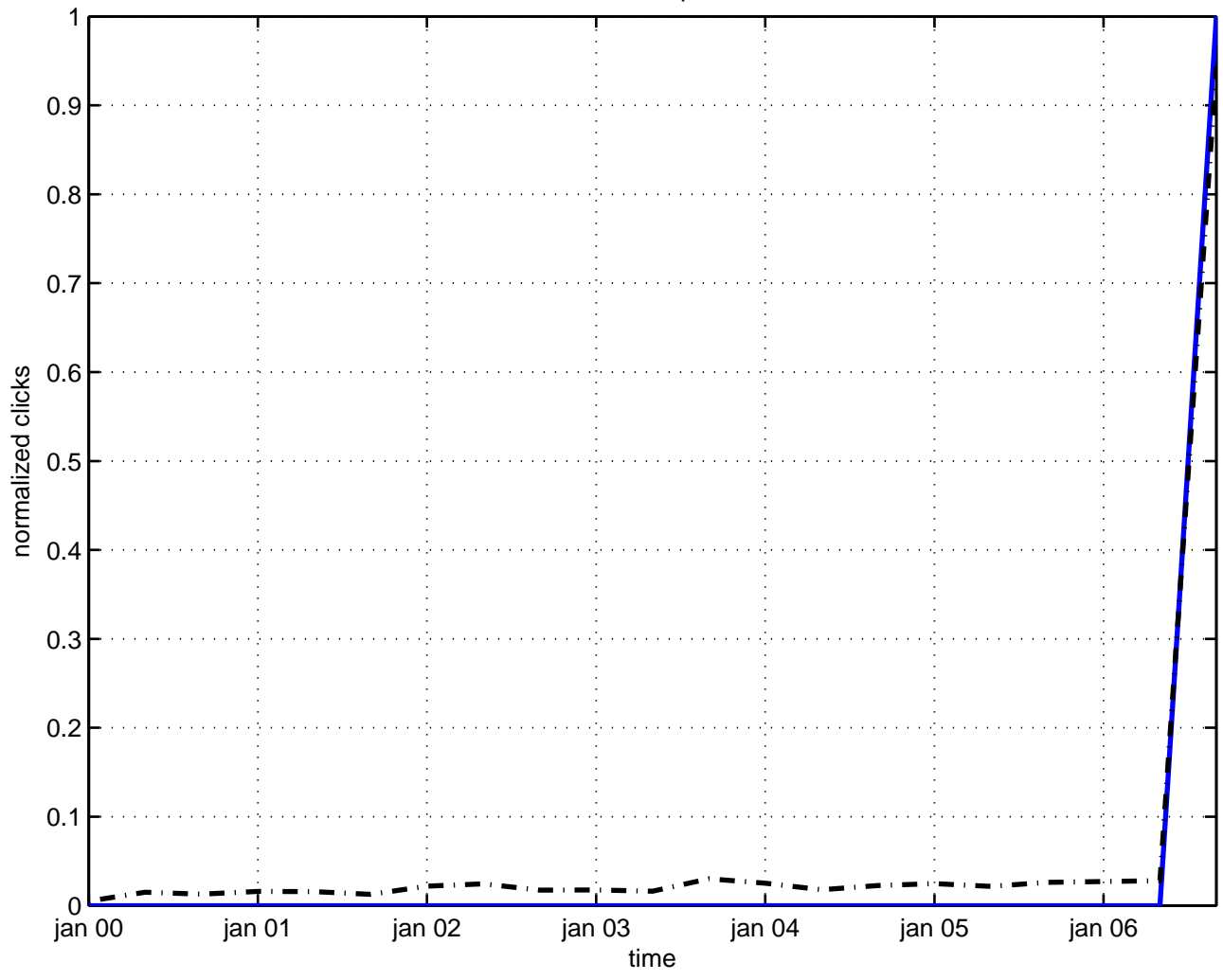
relativistic expansion
